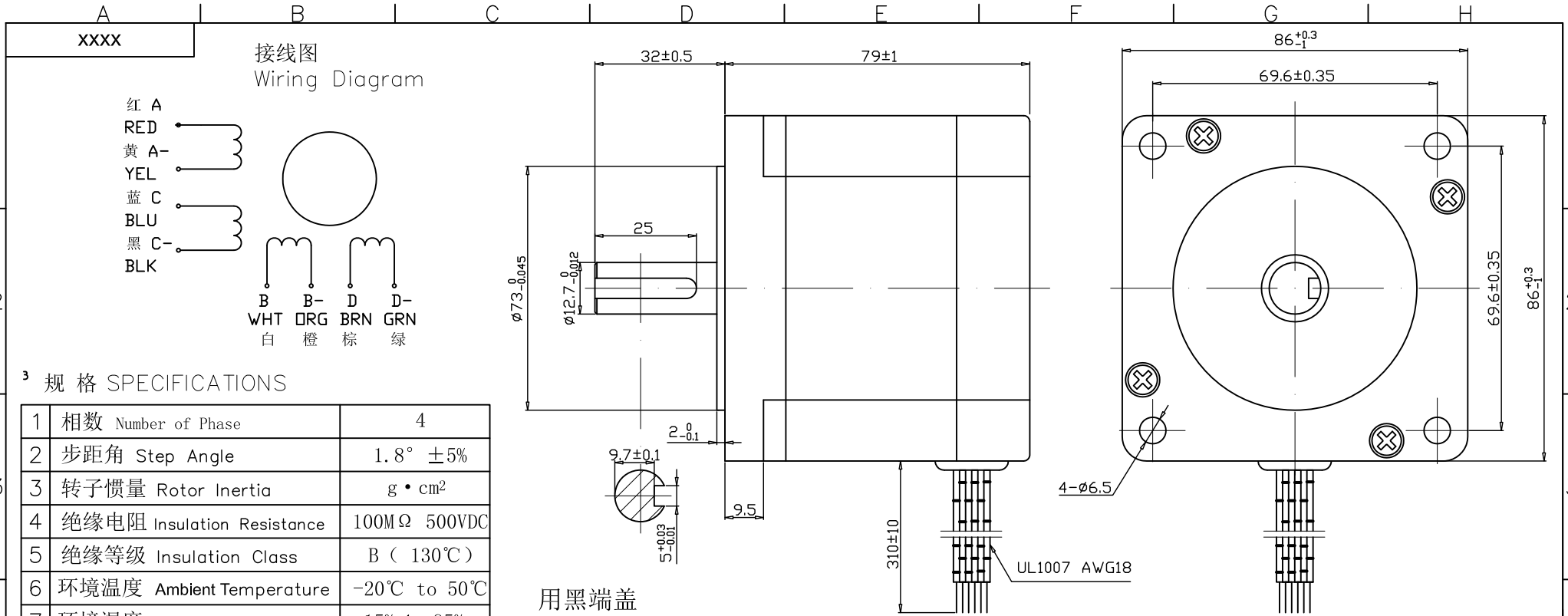
WIRINGS CONNECTION DIAGRAM
